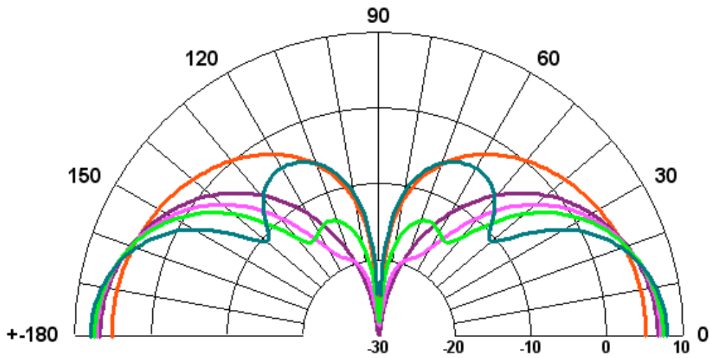
ELEVATION GAIN (dBi) Thin Vertical Radiator over an Infinite, Perfect Ground Plane
