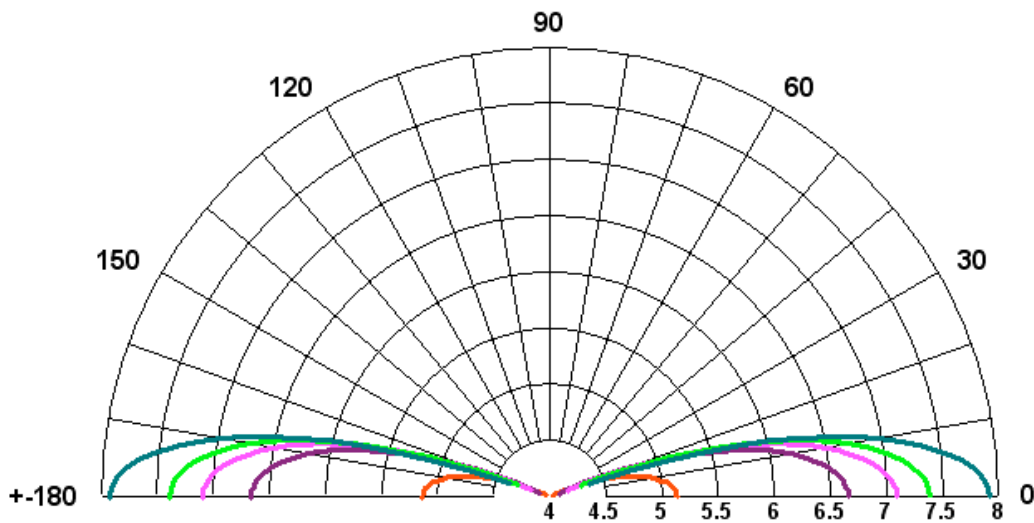
ELEVATION GAIN (dBi) Thin Vertical Radiator over an Infinite, Perfect Ground Plane - Peak Gain Detail -
